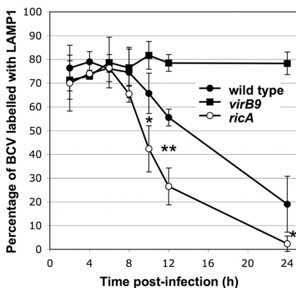
Fig. 7. Trafficking of B. abortus 2308 and its \Delta ricA and \Delta virB9 isogenic mutants. HeLa cells infected with wild-type B. abortus , \Delta ricA mutant and \Delta virB9 mutant were fixed at different time points of the infection. The percentage of wild type, \Delta ricA or \Delta virB9 mutant-containing vacuoles retaining LAMP1, a marker of late endosome, was scored using immunofluorescence microscopy. Data are means \pm standard deviations of three independent experiments. The difference between wild-type strain and \Delta ricA mutant is statistically significant ( P < 0.05 or P < 0.01 for comparisons indicated by * or **, respectively) according to a t -test for independent samples. Complementation of the \Delta ricA mutant in trans is described in the main text.
